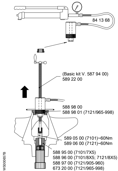
Рис. 47: P7101, P7121
